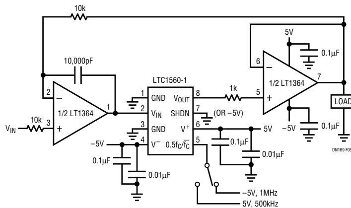
Figure 5. A DC Accurate 500kHz/1MHz Elliptic Filter with an Output Buffer for Driving Cables or Capacitive Loads
